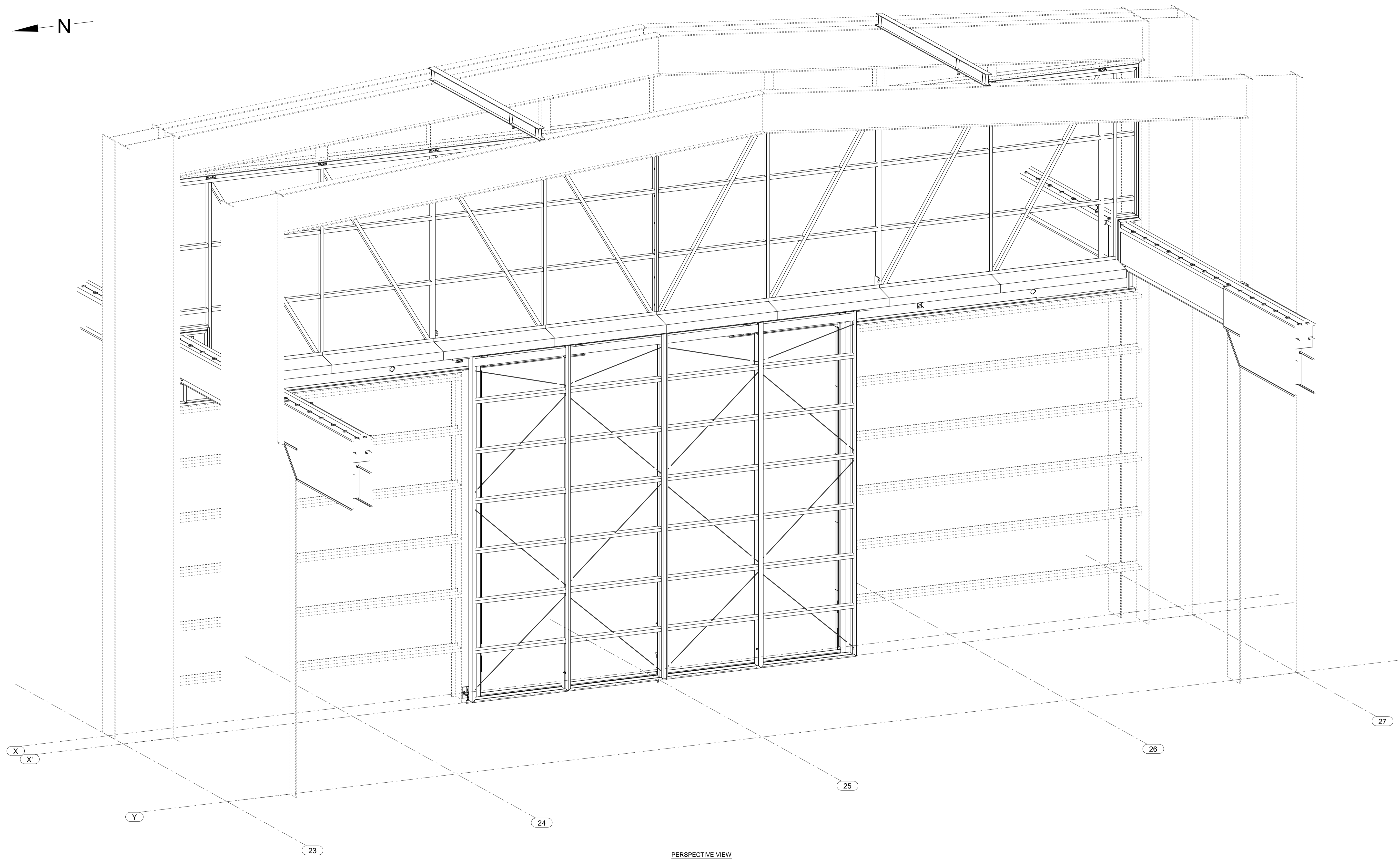
PERSPECTIVE VIEW
